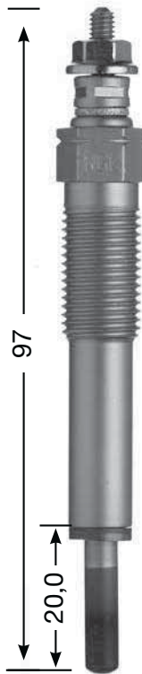
Y-971 M M 12 x 1.25 12 Hex 23 V
