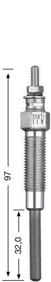
Y-118 T1 M 10 x 1.25 12 Hex 11 V
