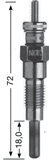
Y-752 M M 12 x 1.25 12 Hex 23 V
